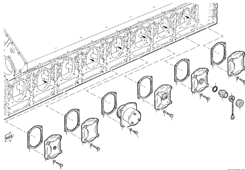
INSPECT PORT COVER 010.00325
