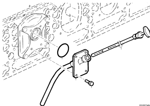
OIL DIPSTICK 010.00347
