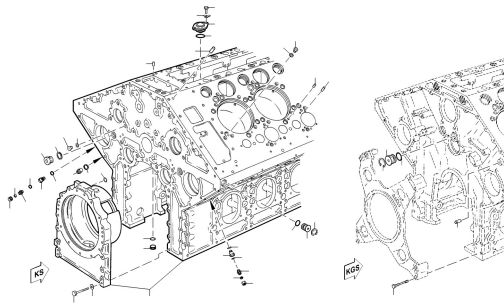
CRANKCASE 010.00323
